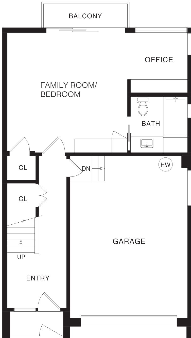
LOWER LEVEL
